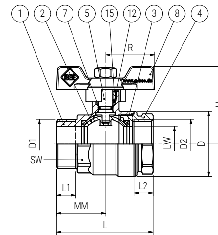
Maßskizze measured sketch
